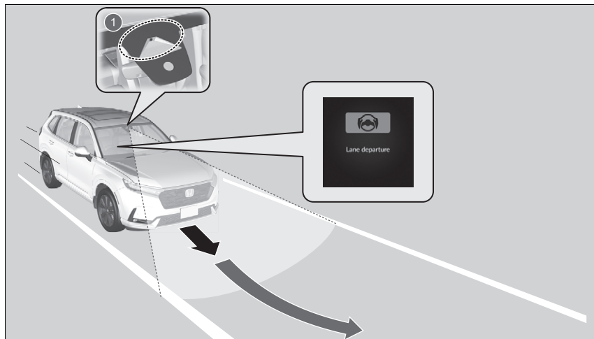
1 Front Sensor Camera: Monitors the lane lines
